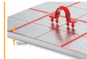
Grapa PS 10/16.
